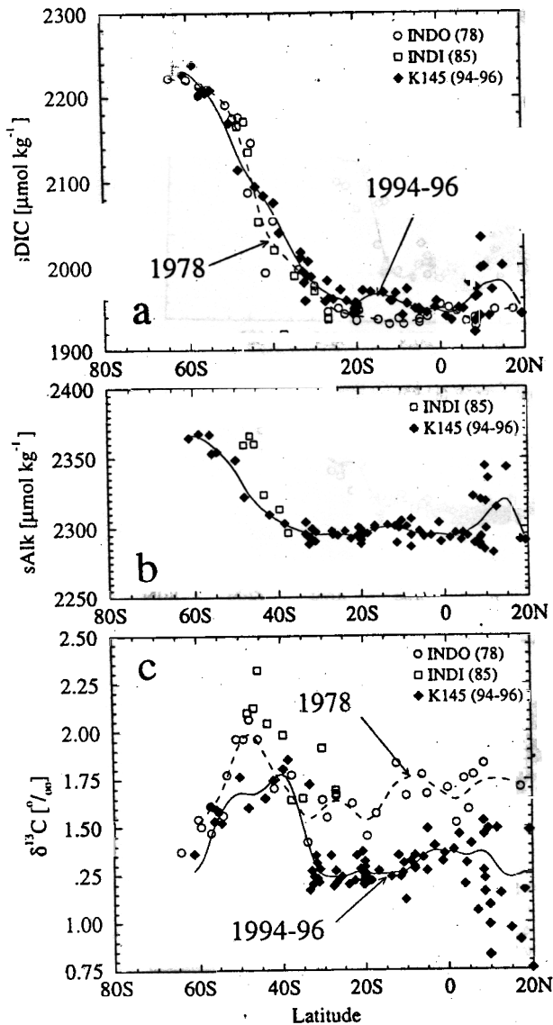
Figure 4. Same as Figure 2, except for the Indian Ocean. Shown are the combined results of 3 programs which span the period from 1978 to 1996. Station locations are given in Figure 1d. For sDIC (a) and \delta^{13}C (c), two spline fits are shown to represent the change between the GEOSECS program in 1978 (solid curve) and the WOCE program in 1994-1996 (dashed curve). North of 30^{\circ}S , a mean difference of 11 \pm 9 \mu\text{mol kg}^{-1} is found for sDIC , and a mean difference of -0.34 \pm 0.07\text{‰} is found for \delta^{13}C . No difference could be calculated for Alk because this quantity has not been measured during GEOSECS. These long term changes reflect the addition of isotopically light anthropogenic CO_2 to the surface ocean ( ^{13}C Suess effect).
