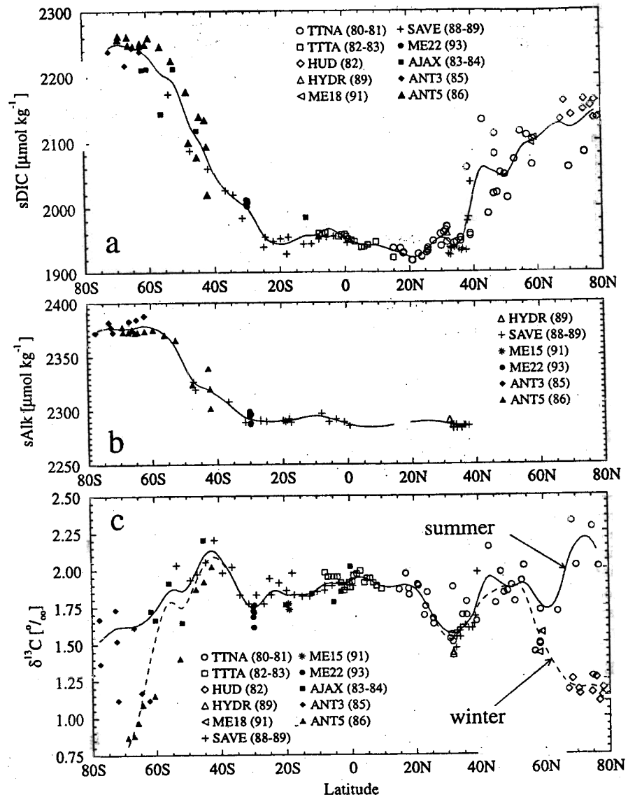
Figure 2. Meridional profiles of inorganic carbon system properties in the upper 50 m of the Atlantic Ocean: (a) normalized dissolved inorganic carbon (sDIC), (b) normalized titration alkalinity (sAlk), and (c) the reduced ^{13}\text{C}/^{12}\text{C} ratio of dissolved inorganic carbon ( \delta^{13}\text{C} ). Shown are the combined results of 11 cruises which span the period from 1980 to 1993. Station locations are given in Figure 1a. Smoothing spline fits have been added to emphasize the trends. For \delta^{13}\text{C} (Figure 2c), two spline fits are shown to represent summer (solid curve) and winter trends (dashed curve) in the high latitudes.
