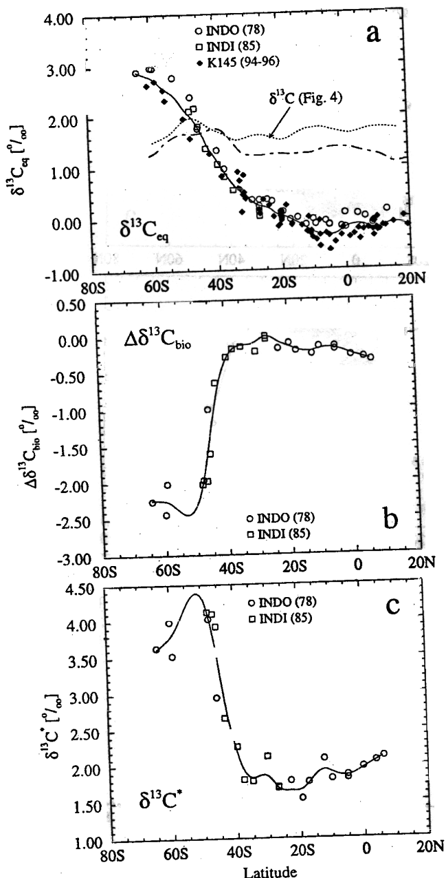
Figure 7. Same as Figure 5, but for the Indian Ocean. The spline fits through the \delta^{13}C observations shown in Figure 4a have been repeated in Figure 7a. In the case of INDO, Alk has been estimated from the global relationship of Gruber et al. [1996] in order to calculate \delta^{13}C_{eq} , \delta^{13}C_{bio} , and \delta^{13}C^* .
