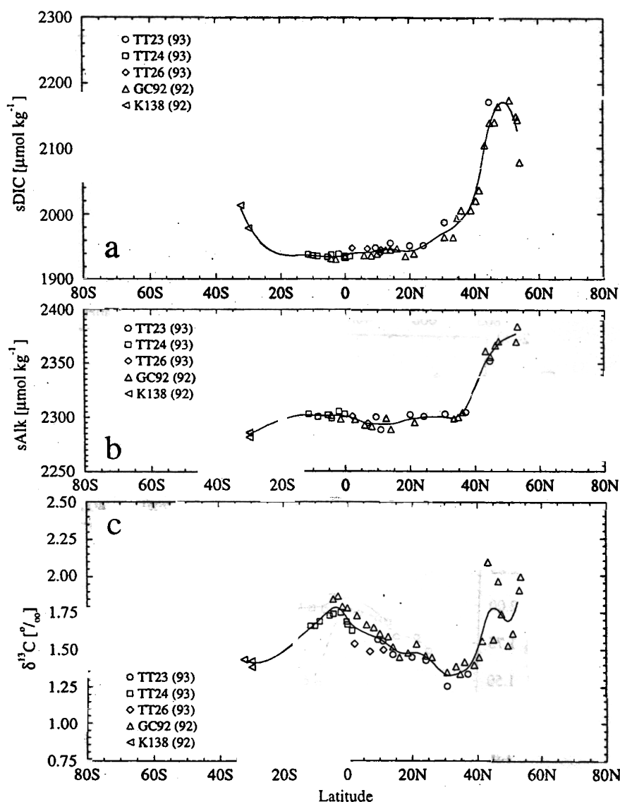
Figure 8. Meridional profiles of inorganic carbon system properties in the upper 50 m of the Western Pacific Ocean (west of 180°E): (a) normalized dissolved inorganic carbon (sDIC), (b) normalized total alkalinity (sAlk), and (c) the ^{13}\text{C}/^{12}\text{C} ratio of dissolved inorganic carbon ( \delta^{13}\text{C} ). Shown are the combined results of five programs which span the period from 1992 to 1993. Station locations are given in Figure 1b. Smoothing spline fits have been added to emphasize the trends.
