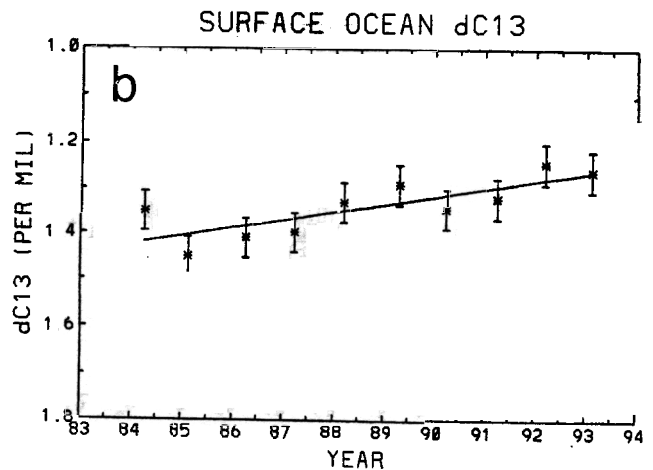
Figure 5b. Daily averages of \delta^{13}\text{C} (‰) associated with the minimum temperature measurement during the year, adjusted for interannual variation by the spline part of the fit described above for Figure 5a. The curve is the straight line part of the fit. The slope of the line is -0.018 \pm 0.005 \text{ ‰ yr}^{-1} .
