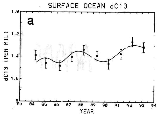
Figure 5a. Daily averages of \delta^{13}\text{C} (‰) associated with the minimum temperature measurement during the year, fit by a constant times the spline of Figure 2 plus a straight line.
