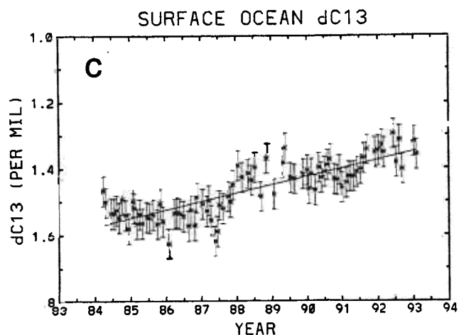
Figure 6c. Daily averages of \delta^{13}\text{C} (‰), seasonally adjusted by the 12- and 6-month period harmonics described above for Figure 6a and adjusted for interannual variation by the (fitted) constant times the temperature spline of Figure 2. The curve is the straight line part of the fit. The slope of the line is -0.025 \pm 0.002 ‰ \text{yr}^{-1} . For convenience in plotting, the data and curve were both adjusted so as to agree with Figure 6b at the year 1988.
