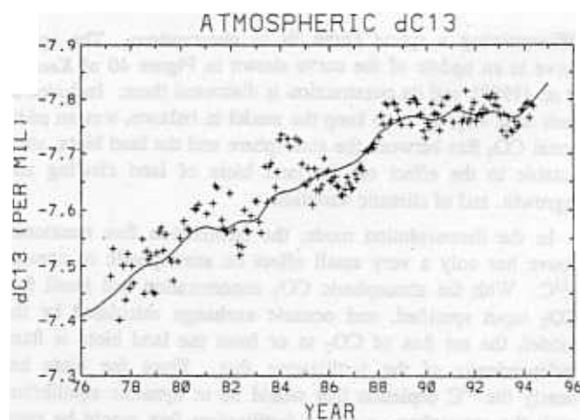
Figure 13. Atmospheric \delta^{13}\text{C} measurements at Mauna Loa, Hawaii, and the south pole. The curve is a prediction from the box diffusion model describe in the text with a diffusivity K of 4000 \text{ m}^2 \text{yr}^{-1} and variation of surface water temperature according to data of Jones et al. [1986a, 1986b, and personal communication, 1994].
