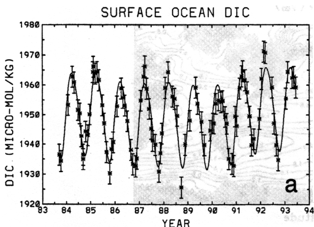
Figure 7a. Daily averages of dissolved inorganic carbon ( \mu\text{mol kg}^{-1} ), fit by a Reinsch-type spline plus harmonics with 12- and 6-month periods. The error per point to produce this fit is 3.5 \mu\text{mol kg}^{-1} .
