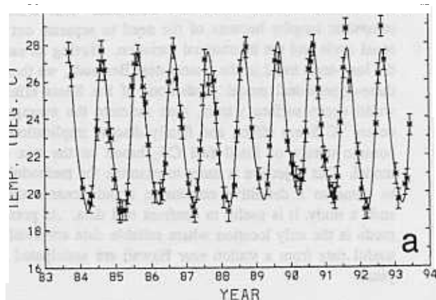
Figure 3a. All temperature measurements at Station S associated with \delta^{13}\text{C} measurements ( ^{\circ}\text{C} ), fit by a Reinsch-type spline plus harmonics with 12- and 6-month periods. The error per point to produce this fit is 0.55^{\circ}\text{C} .
