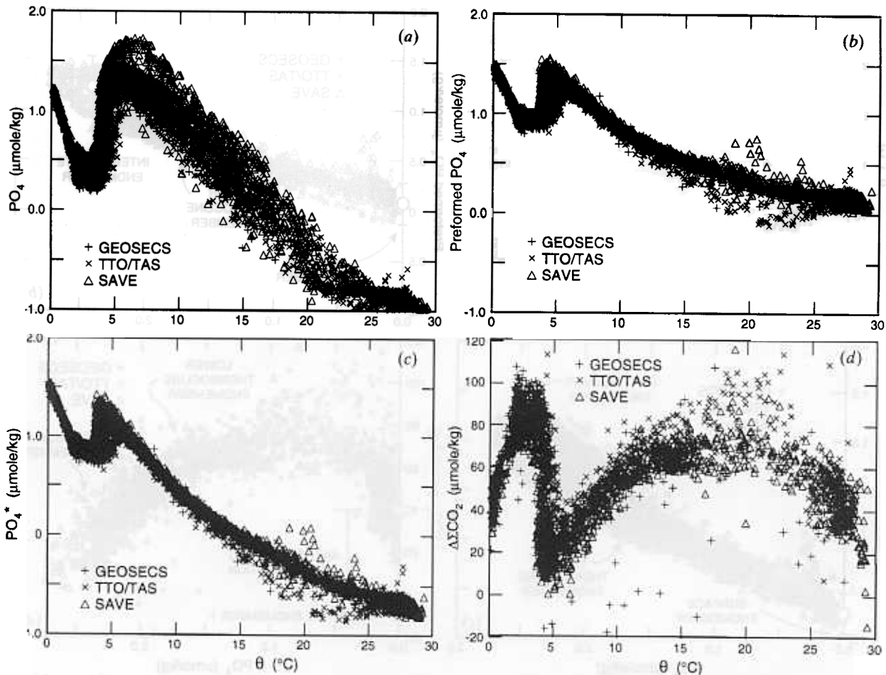
Figure 4. Results from GEOSECS, TTO/TAS and SAVE expeditions for stations between 15°S and 15°N. (a) PO 4 versus \theta ; (b) preformed PO 4 versus \theta ; (c) PO 4 * versus \theta ; (d) \Delta CO 2 versus \theta .
