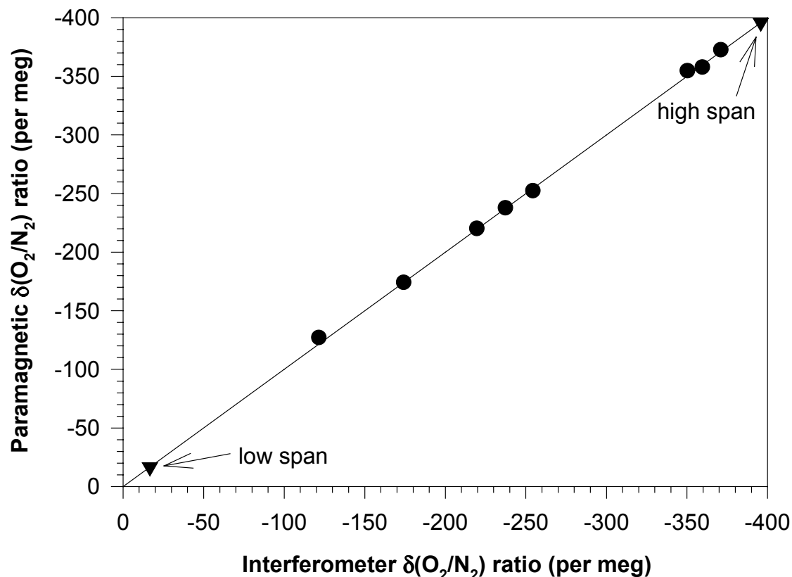
Figure 3.2. Results from a test on the linearity of the response of the paramagnetic analyzer for the range of \text{O}_2/\text{N}_2 ratios expected in ambient air. The solid line is x = y . Triangles indicate the paramagnetic “high span” and “low span” cylinders, which were used to define the span of the analyzer, hence they were forced to be equal to the interferometer-defined ratios. The ratios of the other eight cylinders were then determined from this span.
