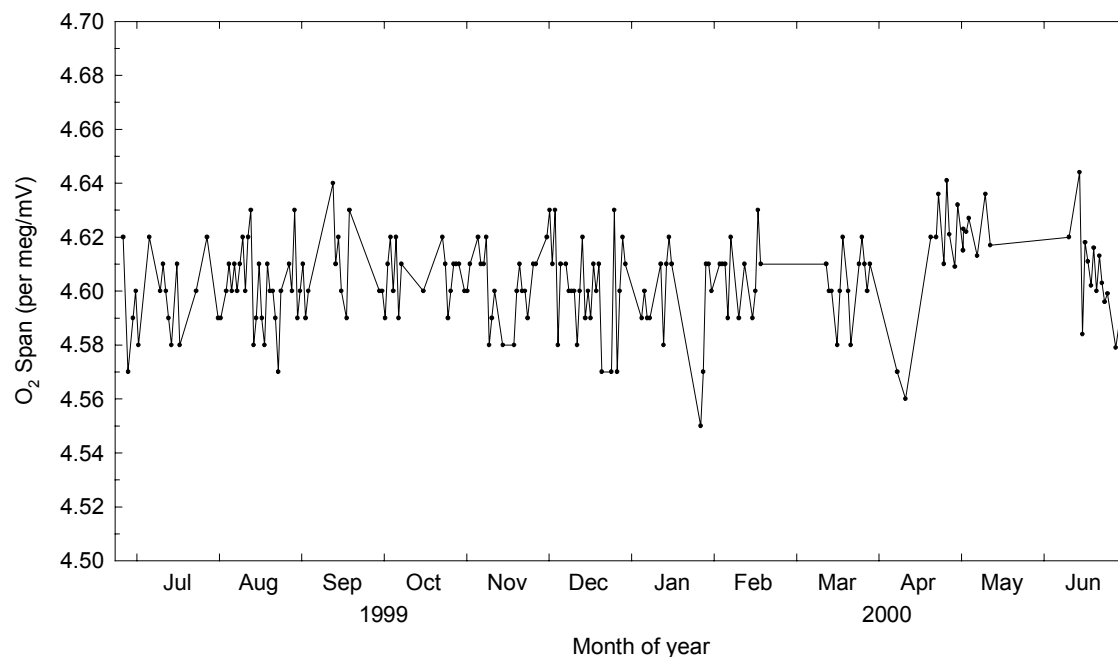
Figure 4.7. Paramagnetic O 2 analyzer span, in units of per meg/mV, calculated daily from the calibration with the high span and low span cylinders. The range of the analyzer span over a full year of operation is less than 2% of the average. Note that the span was reported to only two decimal places prior to 22 April 2000, accounting for the apparent discretized nature of changes in span from day to day prior to this date.
