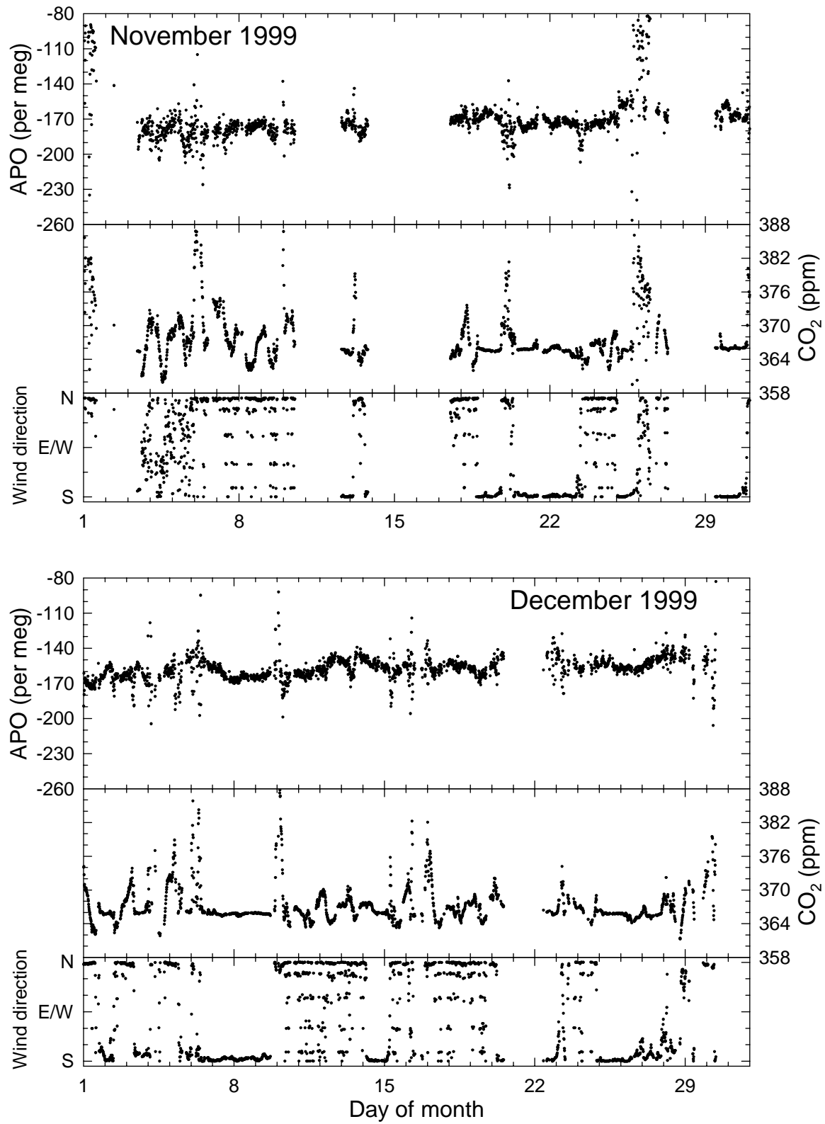
Figure 4.13c. APO, CO 2 and wind direction at Baring Head for November and December 1999.
