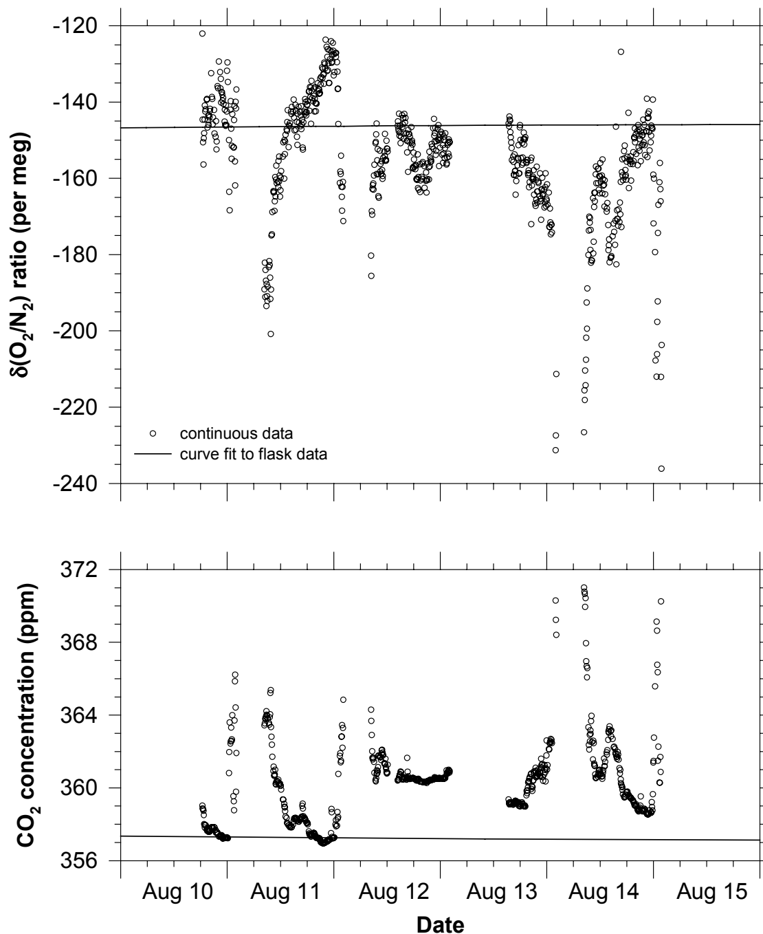
Figure 3.3. Continuous O_2/N_2 and CO_2 measurements sampled from the end of the Scripps Pier for a 1-week period in August 1996. The y axes have been scaled so that O_2/N_2 and CO_2 changes can be compared visually on a mole to mole basis. Data points shown are 2.5-min averages, with one point every 5 min. Gaps in the data are during 4-hourly daily calibration runs or downtime for other logistical reasons. Also shown are the curve fits to the La Jolla flask data (collected at approximately 2 week intervals and analyzed on the interferometric oxygen analyzer), based on a four harmonic seasonal cycle and a stiff spline interannual trend.
