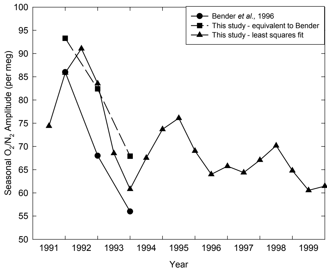
Figure 2.21. Shows the interannual variability in the amplitude of the seasonal cycle observed at Cape Grim. A comparison is made with earlier results from Bender et al. [1996]. Variability has decreased significantly since the early 1990s which the Bender et al. [1996] study examined.
