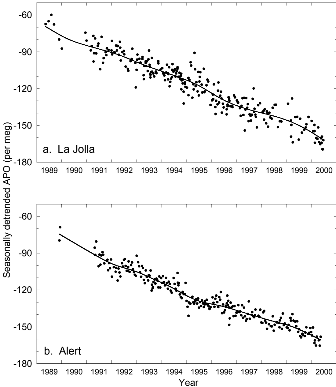
Figure 2.18. Deseasonalized APO data from La Jolla and Alert, used in the computation of global land biotic and oceanic carbon sinks in the 1990s for the IPCC.
