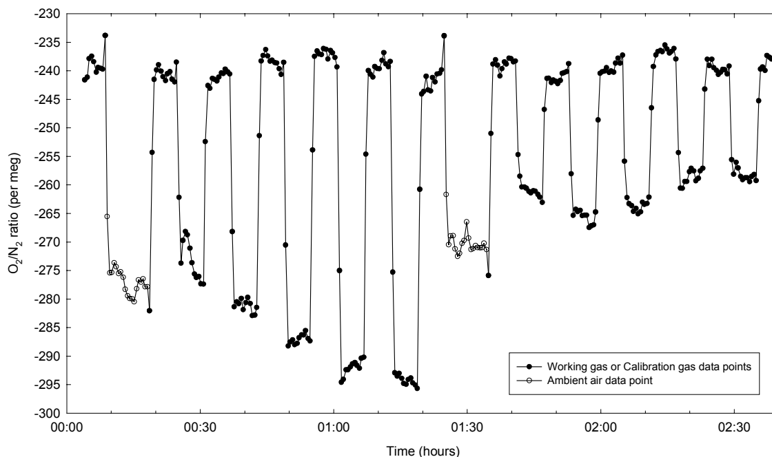
Figure 4.8. Illustrates the pronounced drift in one of the Archive calibration gases, where a downward drift of 25 per meg can be seen from the first to the fifth jog. In comparison, the working gas jogs, at approximately -240 per meg, show much greater stability over time. In contrast to Figures 4.2 and 4.3, data points shown here are not every second, but 30 second averages.
