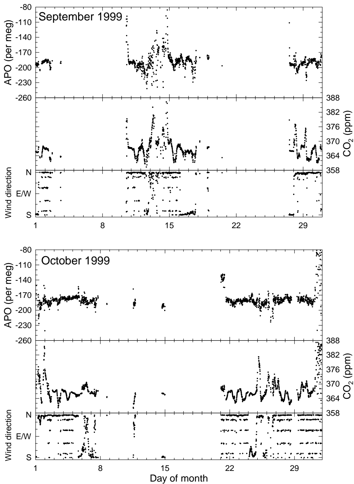
Figure 4.13b. APO, CO 2 and wind direction at Baring Head for September and October 1999.
