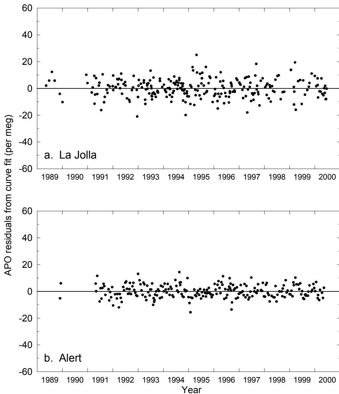
Figure 2.19. APO flask residuals from the curve fits of Figure 2.4 for La Jolla and Alert. These residuals give a measure of the uncertainty to assign in the calculation of global land biotic and oceanic carbon sinks. The figure also shows that early 1989 data are not more variable than more recent parts of the record.
