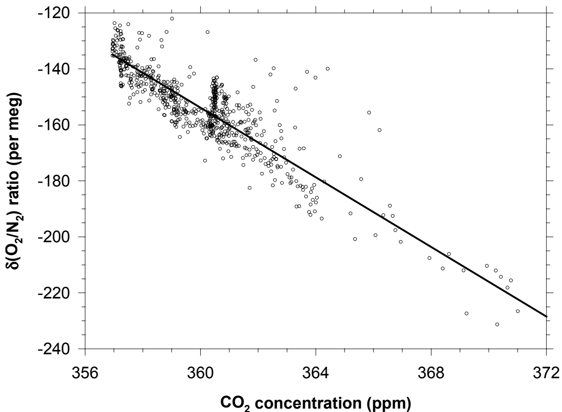
Figure 3.4. O 2 /N 2 and CO 2 data from Figure 3.3 plotted against each other. The correlation is good, with an r^2 of 0.88. The slope of the best-fit line is -6.22 \pm 0.09 per meg/ppm, or 1.30 \pm 0.02 mol O 2 consumed per mol CO 2 produced, close to but lower than a value of 1.44 that would be expected if all the air was polluted by fossil fuel combustion from petroleum based fuels only. The residuals from the linear fit are larger than expected from instrumental imprecision, illustrating that O 2 /N 2 and CO 2 are not always anticorrelated in ambient air.
