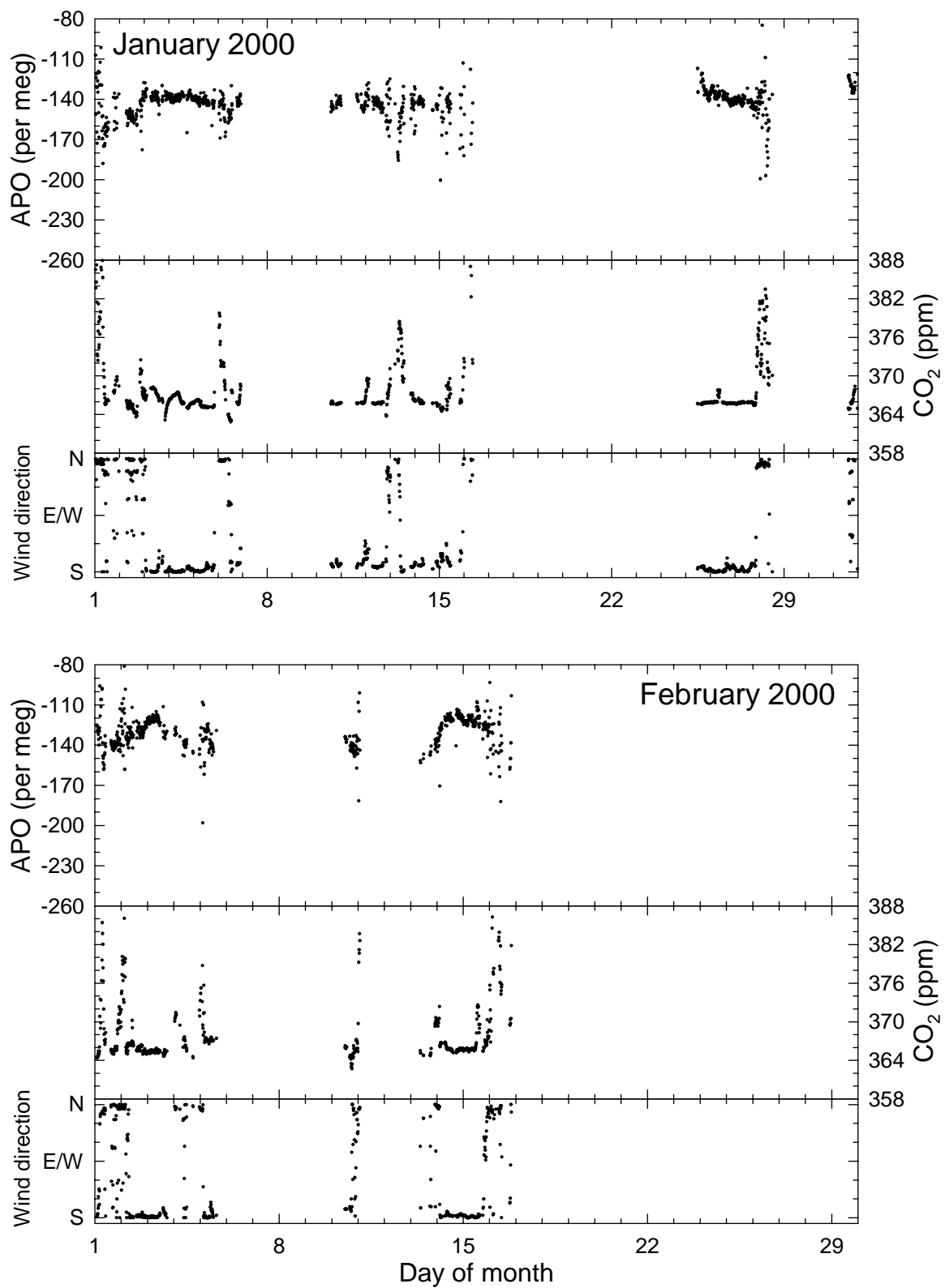
Figure 4.13d. APO, CO 2 and wind direction at Baring Head for January and February 2000.
