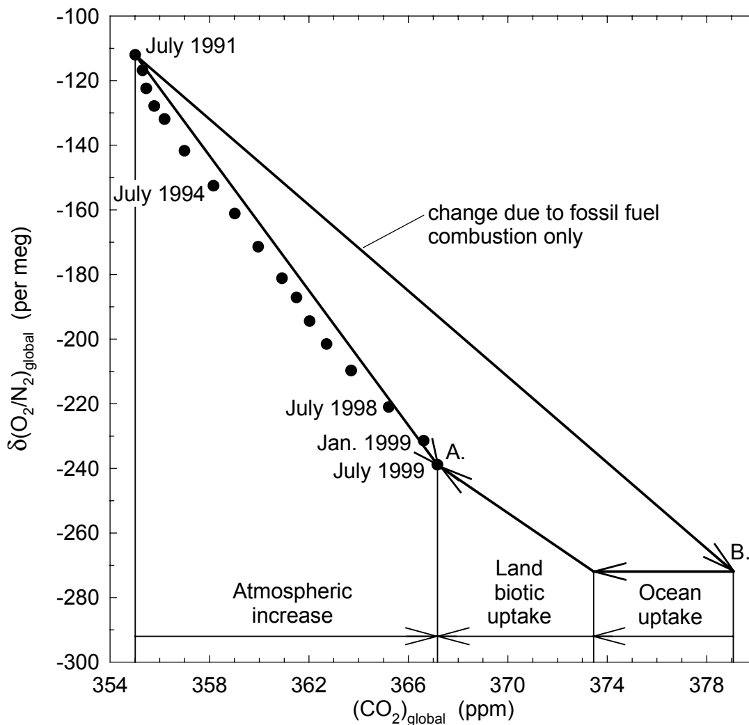
Figure 2.17. Vector diagram showing the calculation of the global land biotic and oceanic carbon sinks. Solid circles are annual averages of the observed O_2 and CO_2 concentrations, calculated from global averages of Alert, La Jolla, and Cape Grim. Also shown is a fossil fuel combustion line, representing the change in atmospheric O_2 and CO_2 concentrations that would have occurred if all CO_2 emitted remained in the atmosphere. The slope for the land biotic sink is fixed to an O_2:C molar ratio of -1.1 , the best estimate of the ratio observed for land photosynthesis and respiration processes, whereas the oceanic sink assumes that there is no effect on O_2 , as described in the text.
