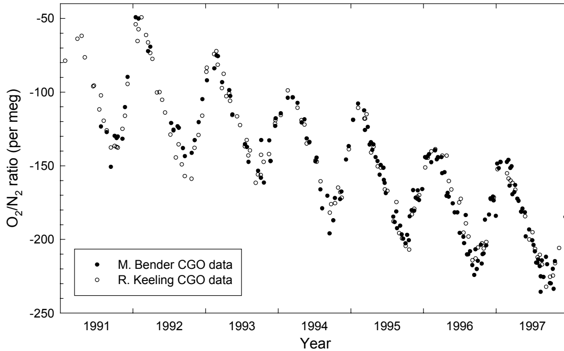
Figure 2.22. O_2/N_2 ratio data from flask samples collected at Cape Grim, Tasmania, Australia, by two independent programs run by M. Bender at Princeton University, and R. Keeling at Scripps Institution of Oceanography. All flask samples are collected by the same station personnel under identical criteria for appropriate sampling conditions.
