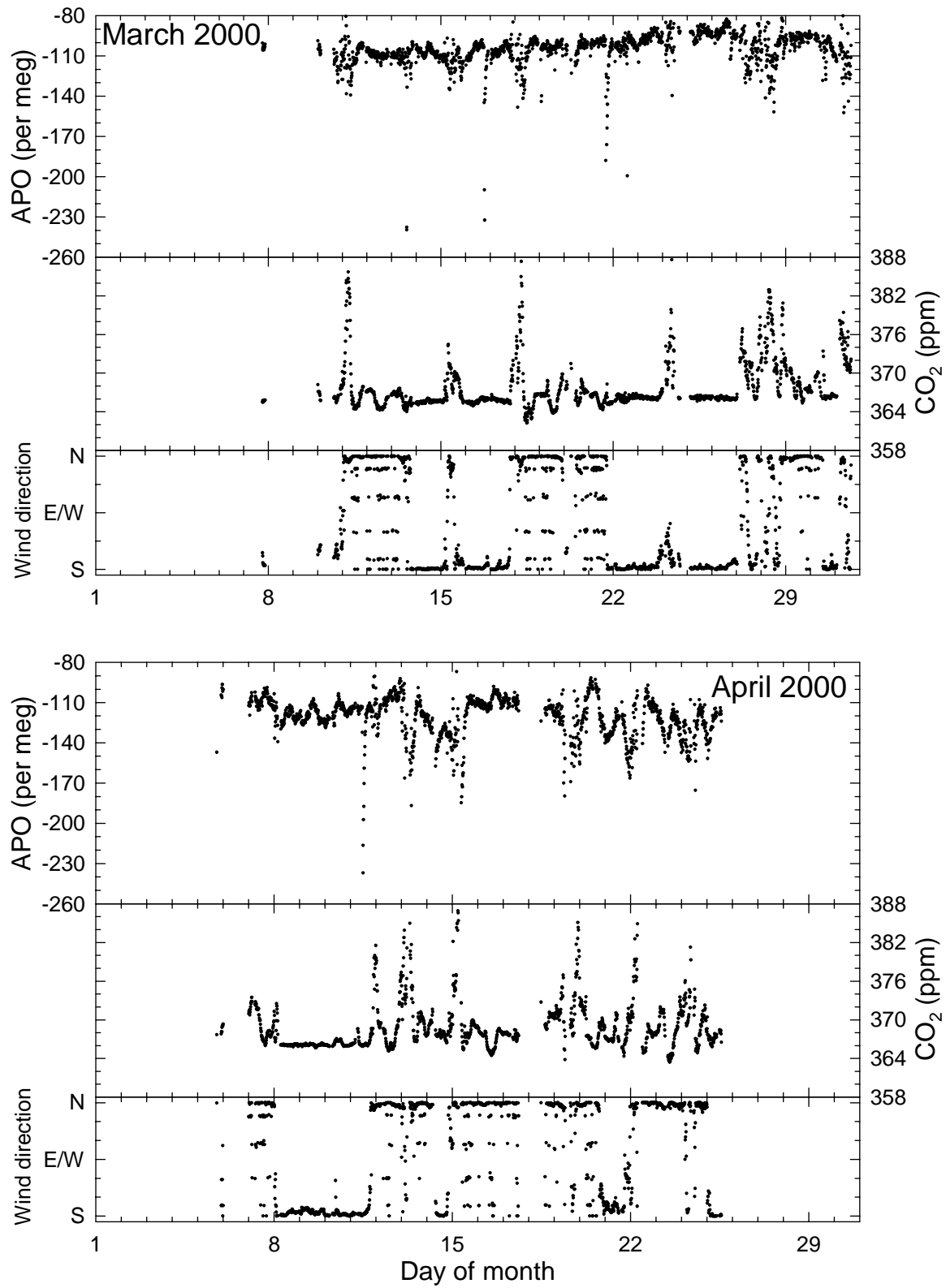
Figure 4.13e. APO, CO 2 and wind direction at Baring Head for March and April 2000.
