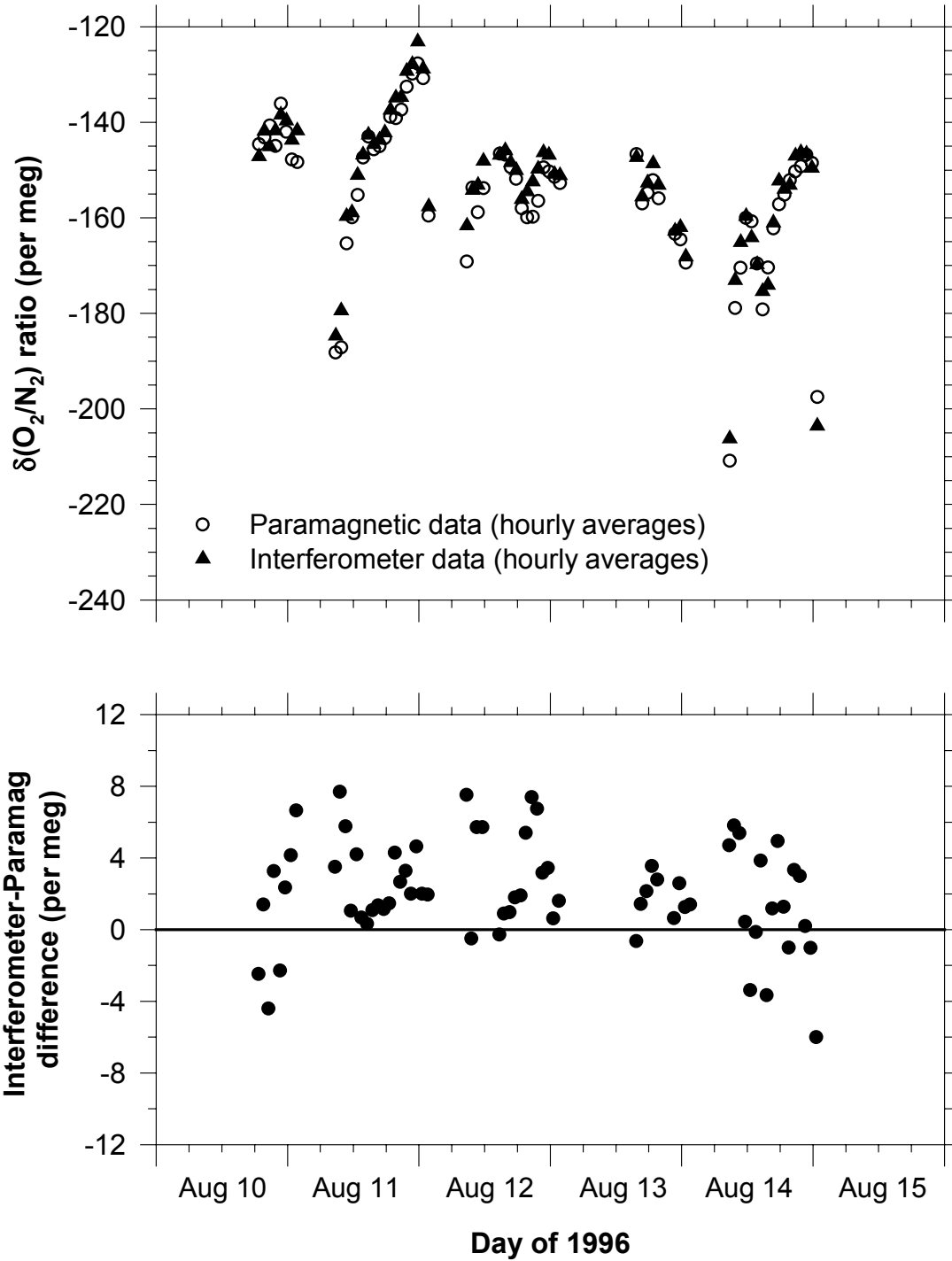
Figure 3.5. For the same period of continuous data collection on the paramagnetic analyzer, concurrent interferometer \text{O}_2/\text{N}_2 ratio data were collected. Apart from a small calibration offset, the two analyzers show the same features with similar precision. Note that the interferometer outputted one data point per hour, so the paramagnetic data were binned and averaged accordingly for this graph.
