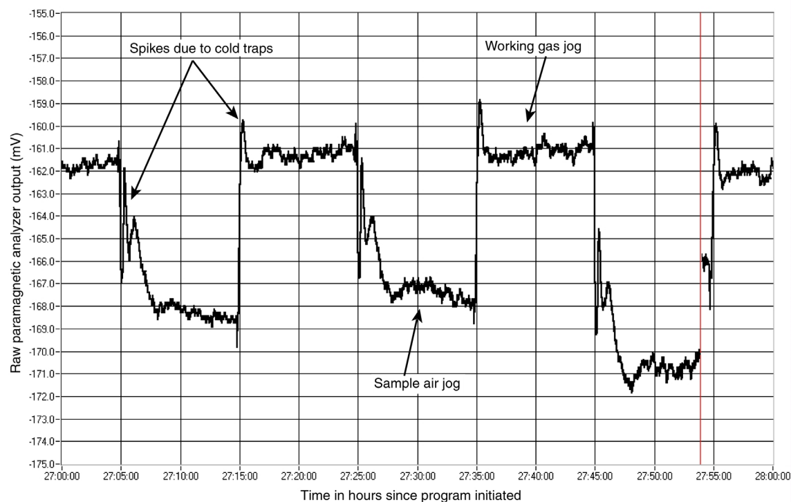
Figure 4.3. As for Figure 4.2, raw analyzer output signal is shown with a data point every second and 1 mV roughly equal to 5 per meg. Thus full scale in this figure is 100 per meg, and one hour of data are shown. This figure illustrates the transient spikes in O 2 concentrations that are caused when valve switching disturbs the O 2 /N 2 ratio gradient equilibrium that is set up in the cryogenic cold traps.
