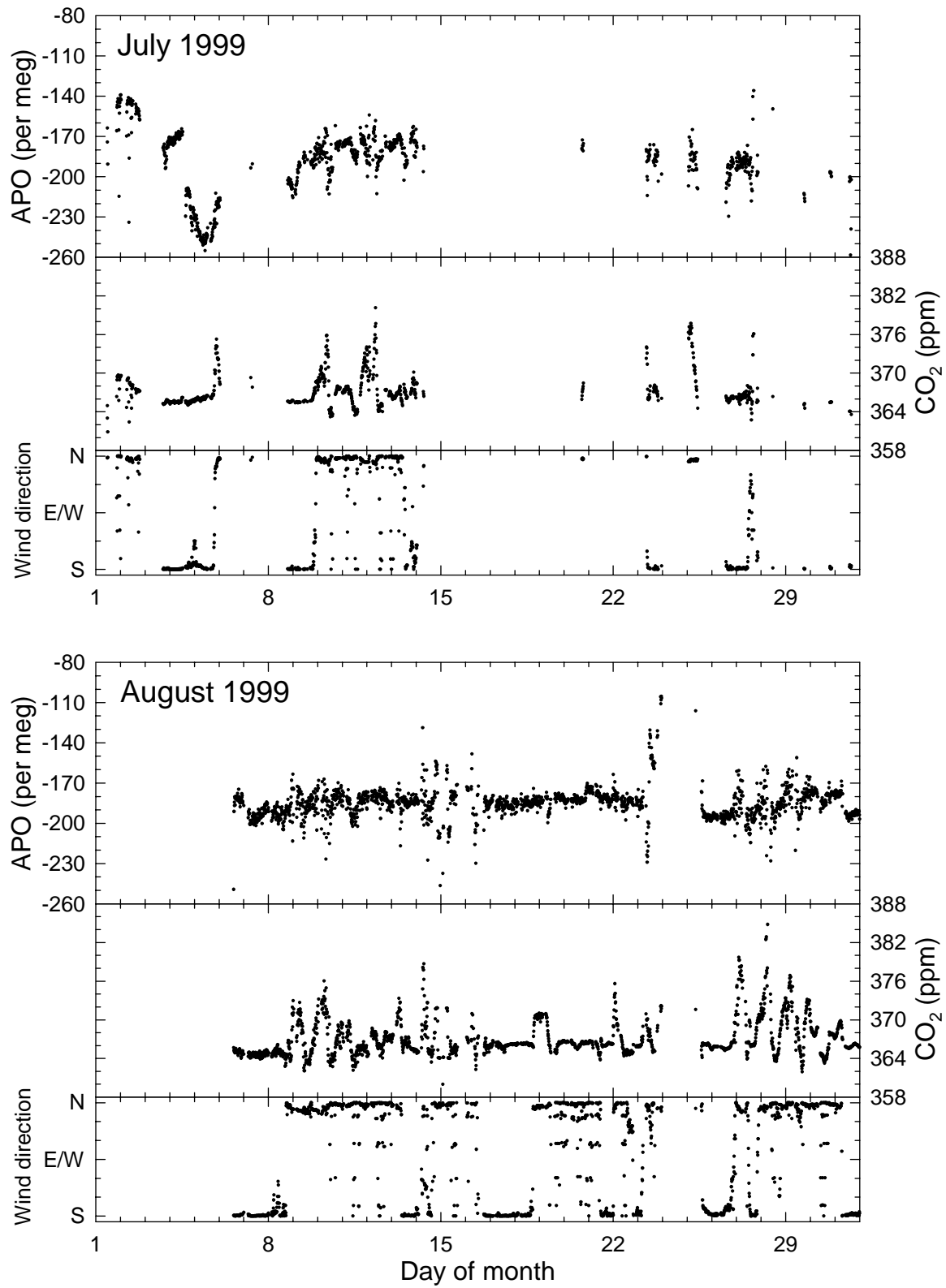
Figure 4.13a. APO, CO 2 and wind direction at Baring Head for July and August 1999. Wind direction is shown as the cosine of the direction in degrees.
