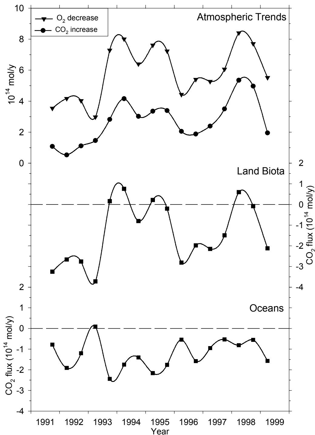
Figure 2.20. Land biotic and oceanic carbon sinks calculated on an annual basis with the same computational technique used in Figure 2.17. The triangles and circles on the top plot show the atmospheric O 2 and CO 2 trends respectively. This plot shows increases of CO 2 to the atmosphere, and decreases of O 2 . Because O 2 changes can not be expressed in units of Gt C/y, all units in this figure are in 10^{14} moles. Throughout the 1990s atmospheric O 2 decreased at a faster rate than CO 2 increased. The land biotic sink exhibits much greater interannual variability than the oceanic sink.
