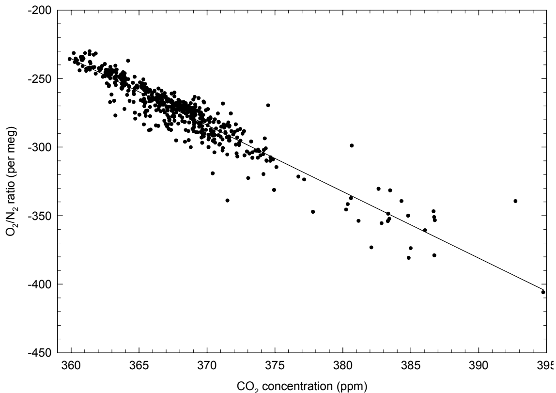
Figure 4.17. Shows the O 2 /N 2 ratio correlation with CO 2 concentration for air arriving at Baring Head from 3-10 November 1999. These data have a slope of 1.13 mol O 2 consumed per mole of CO 2 produced, and have a good r^2 value of 0.91. Wind conditions during this time were persistent northerlies, indicating that the land biota is the main influence driving O 2 /N 2 ratio and CO 2 concentration changes.
