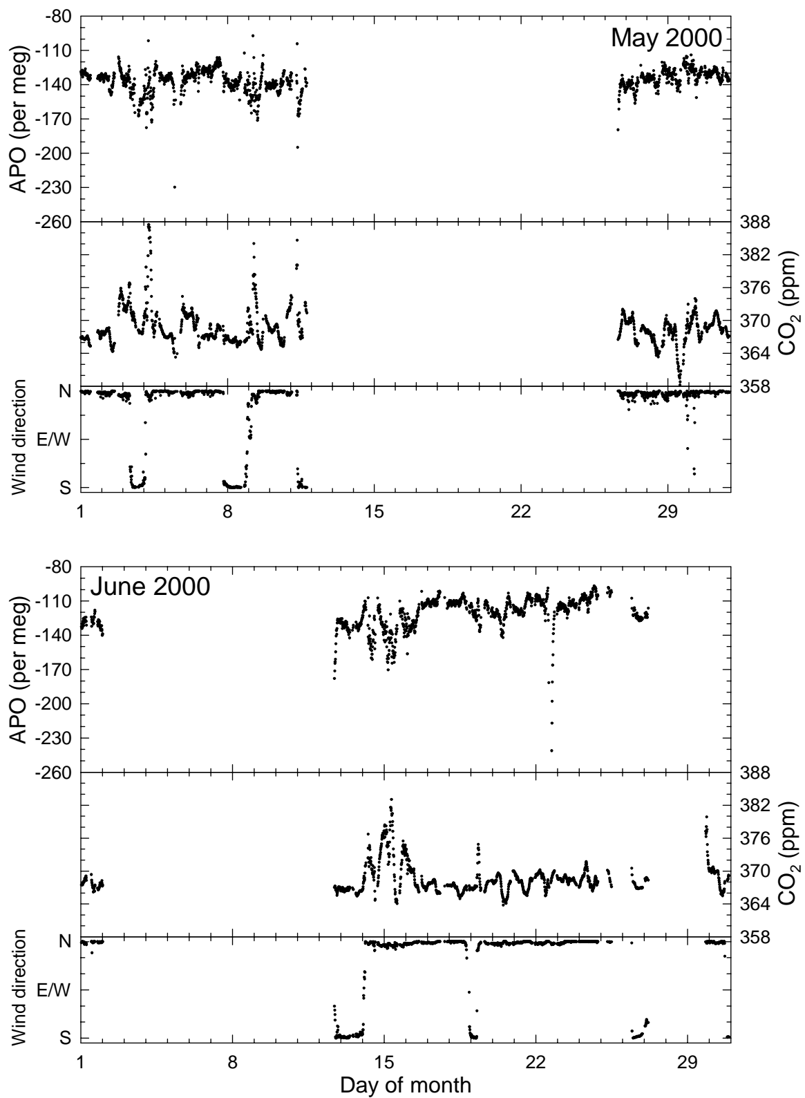
Figure 4.13f. APO, CO 2 and wind direction at Baring Head for May and June 2000.
