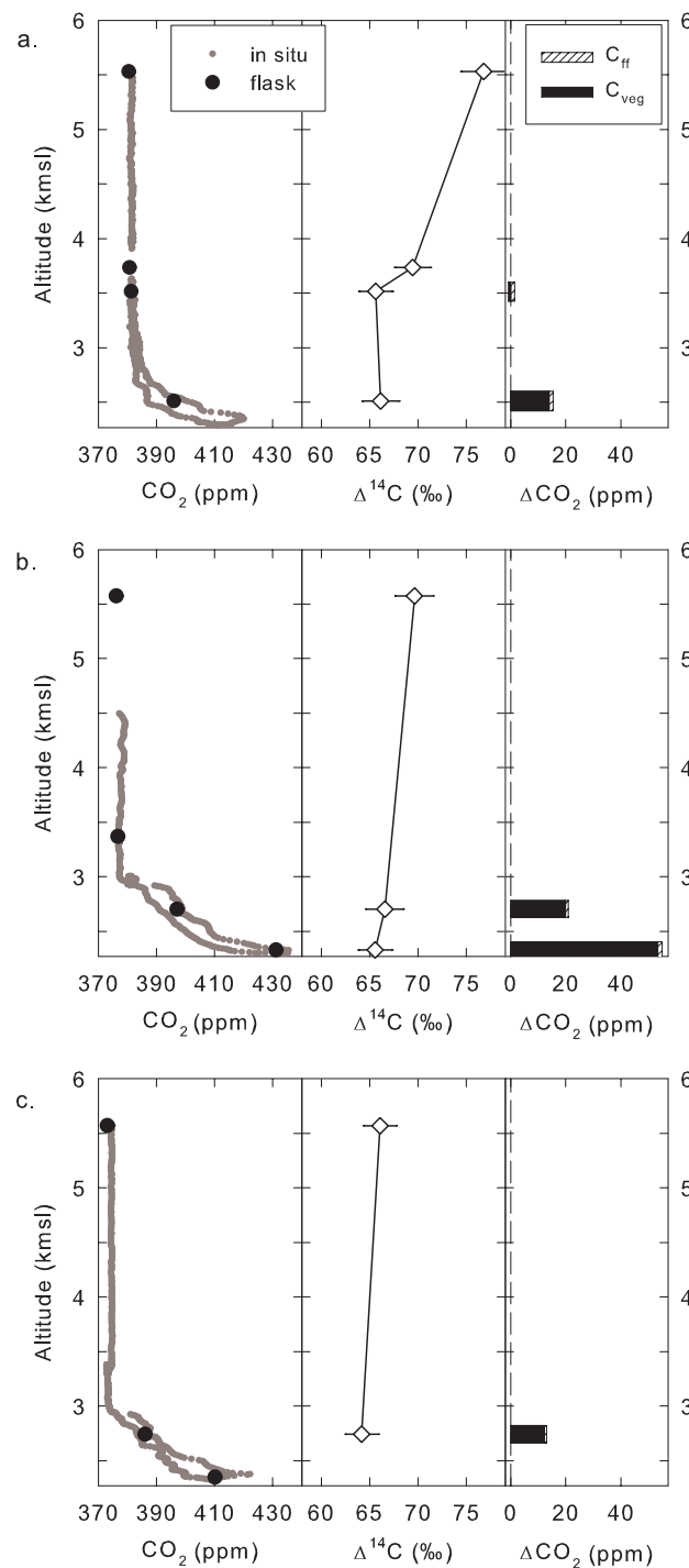
Figure 5.3: Profiles sampled near 7 a.m. in the rural area on a. May 20, 2004, b. July 22, 2004 and c. July 26, 2004. Measured CO 2 concentration (flask data in black circles; in situ data in gray circles), Δ 14 C (diamonds), and the amount of CO 2 added (ΔCO 2 ) as C veg (black bars) and C ff (hatched bars). Altitude is given in km ASL, where the ground level is at the base of the plot (2.27 km ASL).
