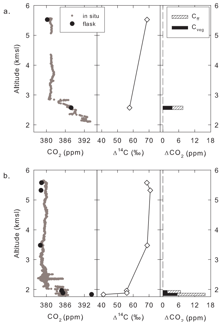
Figure 5.4: Profiles near 10 a.m. sampled in the urban area on a. May 20, 2004 and b. July 20, 2004. Measured CO 2 concentration (flask data in black circles; in situ data in gray circles), Δ 14 C (diamonds), and the amount of CO 2 added (ΔCO 2 ) as C veg (black bars) and C ff (hatched bars). Altitude is given in km ASL, where the ground level is at the base of the plot (1.76 km ASL).
