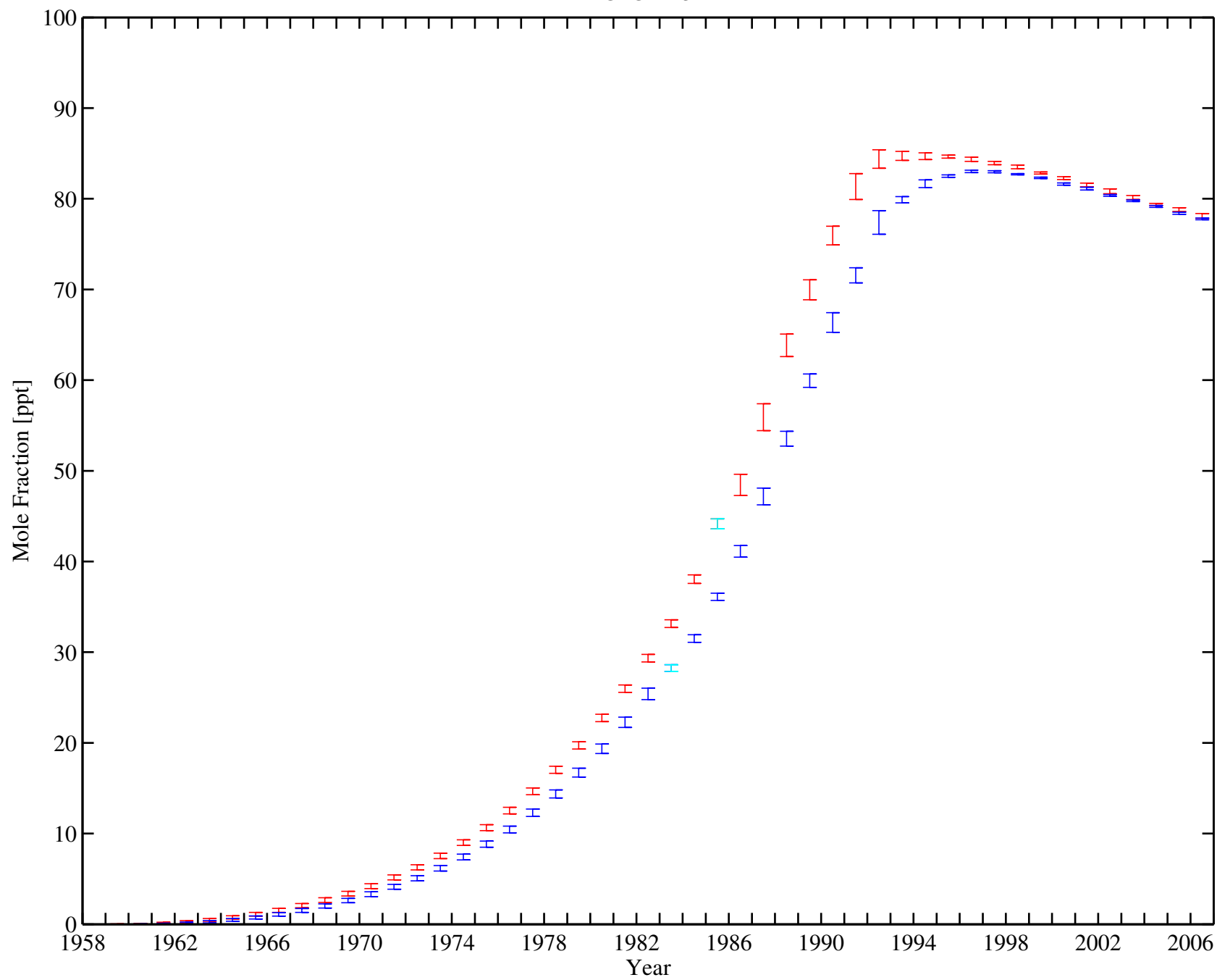
CFC-113
